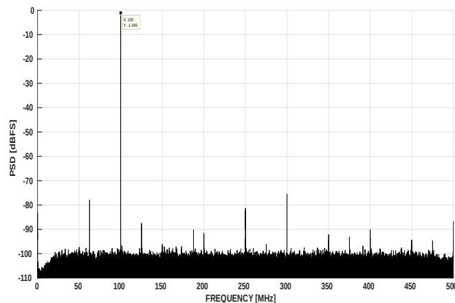
图 7-15. FFT at F_{in} = 100\text{MHz} , 1GSPS (0.8Vpp FS)
