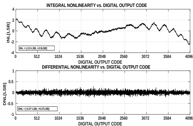
图 7-14. INL/DNL at F_{in} = 100\text{MHz} , 1GSPS (0.8Vpp FS)
