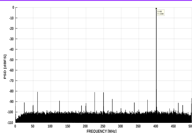
图 7-19. FFT at F_{in} = 400\text{MHz} , 1GSPS (1.0Vpp FS)
