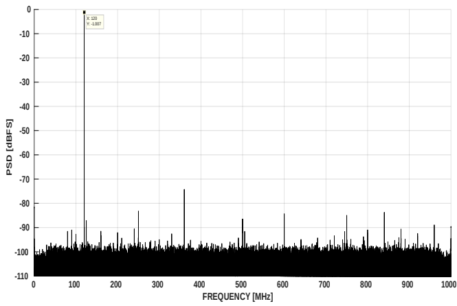
图 7-10. FFT at F_{in} = 120\text{MHz} , 2GSPS (1.0Vpp FS)
