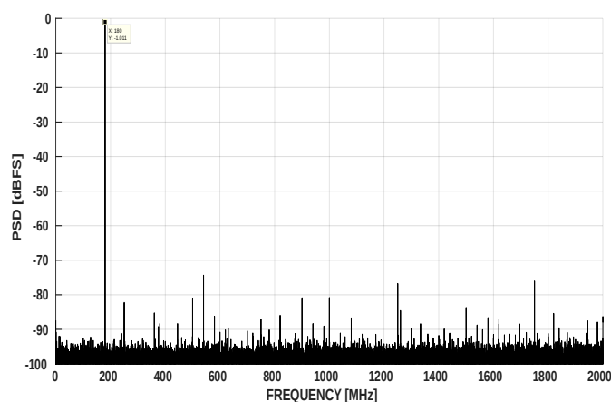
图 7-4. FFT at F_{in} = 180\text{MHz} , 4GSPS (1.0Vpp FS)
