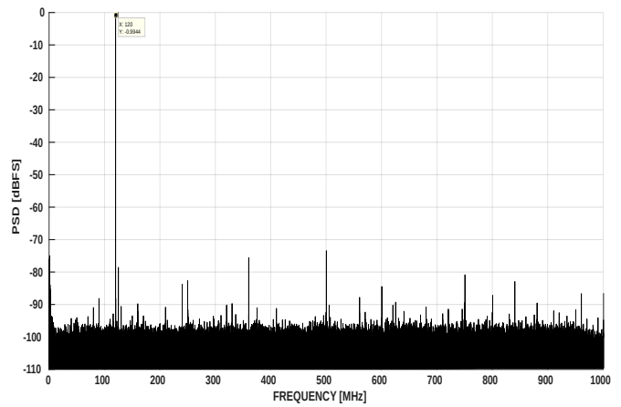
图 7-9. FFT at F_{in} = 120\text{MHz} , 2GSPS (0.8Vpp FS)
