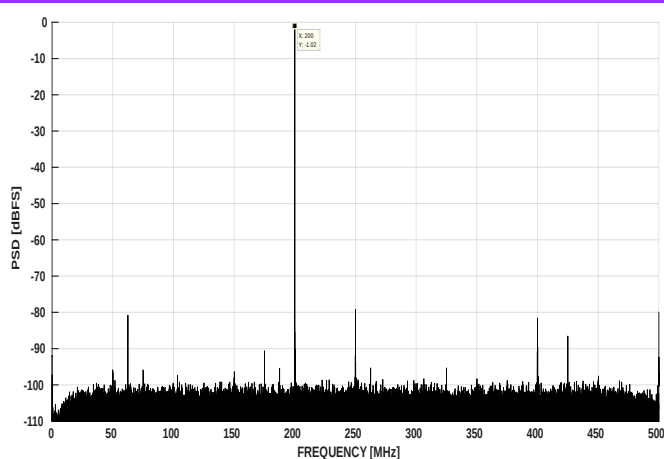
图 7-18. FFT at F_{in} = 200\text{MHz} , 1GSPS (1.0Vpp FS)
