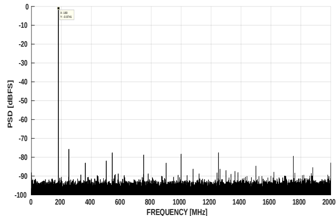
图 7-3. FFT at F_{in} = 180\text{MHz} , 4GSPS (0.8Vpp FS)
