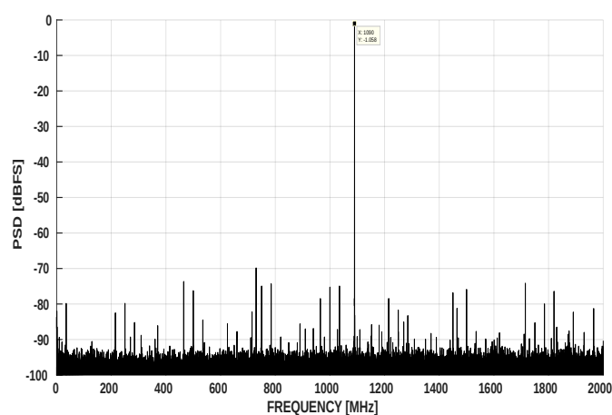
图 7-6. FFT at F_{in} = 1.09\text{GHz} , 4GSPS (1.0Vpp FS)
