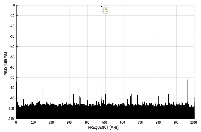
图 7-11. FFT at F_{in} = 480\text{MHz} , 2GSPS (0.8Vpp FS)
