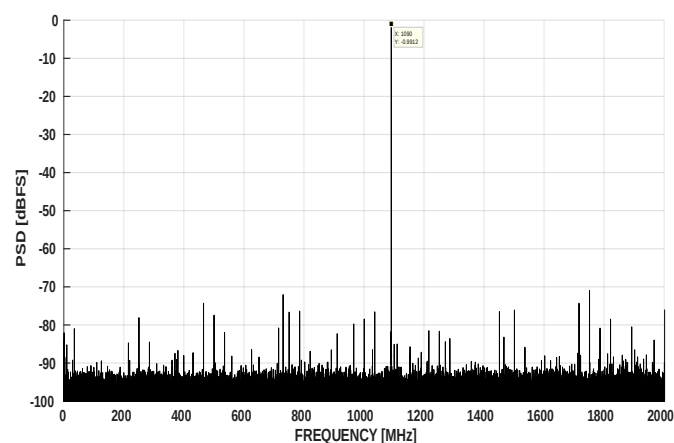
图 7-5. FFT at F_{in} = 1.09\text{GHz} , 4GSPS (0.8Vpp FS)
