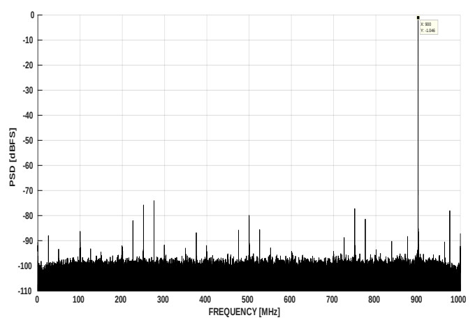
图 7-13. FFT at F_{in} = 900\text{MHz} , 2GSPS (1.0Vpp FS)
