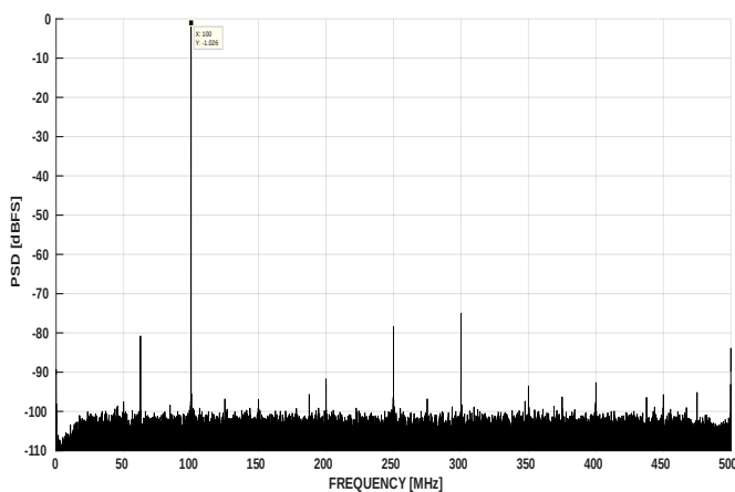
图 7-16. FFT at F_{in} = 100\text{MHz} , 1GSPS (1.0Vpp FS)
