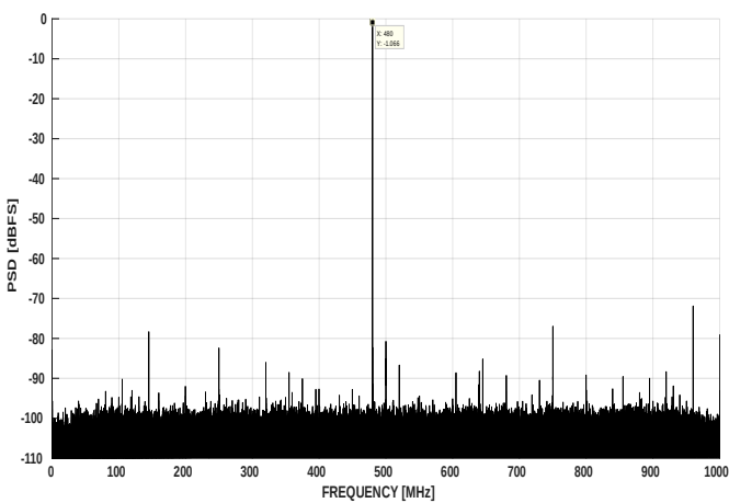
图 7-12. FFT at F_{in} = 480\text{MHz} , 2GSPS (1.0Vpp FS)
