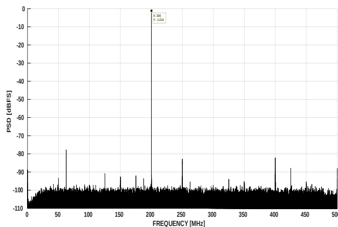
图 7-17. FFT at F_{in} = 200\text{MHz} , 1GSPS (0.8Vpp FS)
