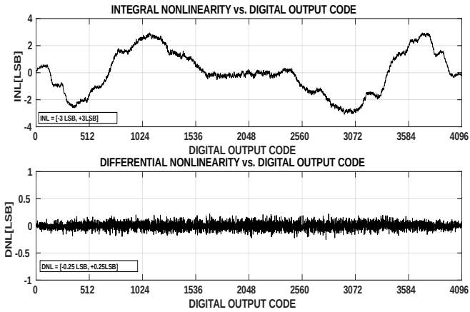
图 7-8. INL/DNL at F_{in} = 100\text{MHz} , 2GSPS (0.8Vpp FS)
