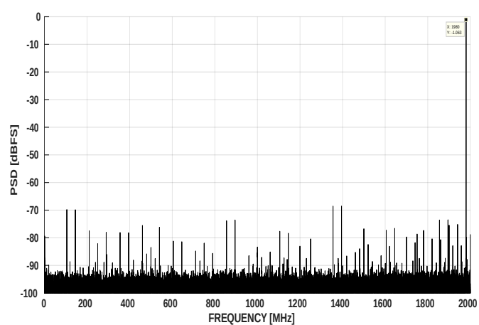
图 7-7. FFT at F_{in} = 1.98\text{GHz} , 4GSPS (1.0Vpp FS)
