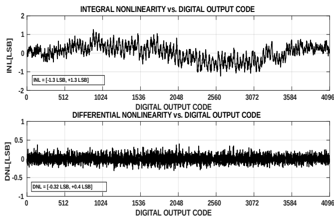
图 7-2. INL/DNL at F_{in} = 180\text{MHz} , 4GSPS (0.8Vpp FS)
